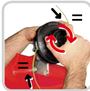
Line loading in 30".
